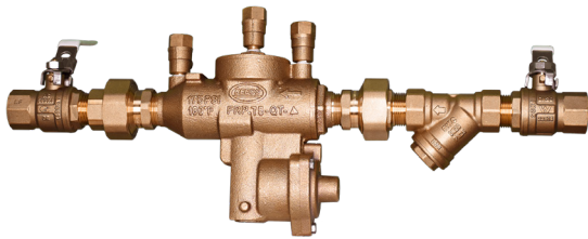
RPZD Backflow Preventers 15mm – 50mm
